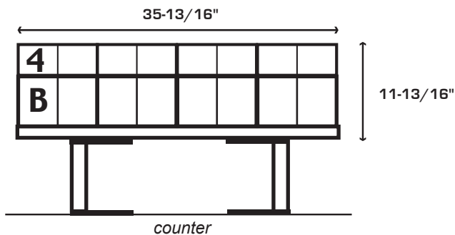
4 Wide Dual Bingo + 4 Wide Dual 4'' #OTS00B44W
