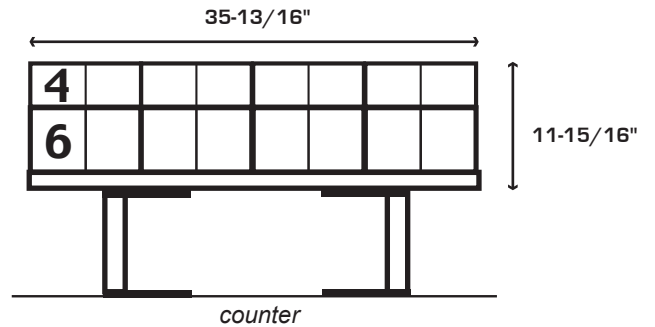
4 Wide Dual 6'' + 4 Wide Dual 4'' #OTS00644W
