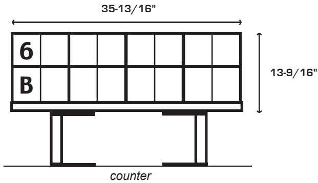
4 Wide Dual Bingo + 4 Wide Dual 6'' #OTS00B64W
