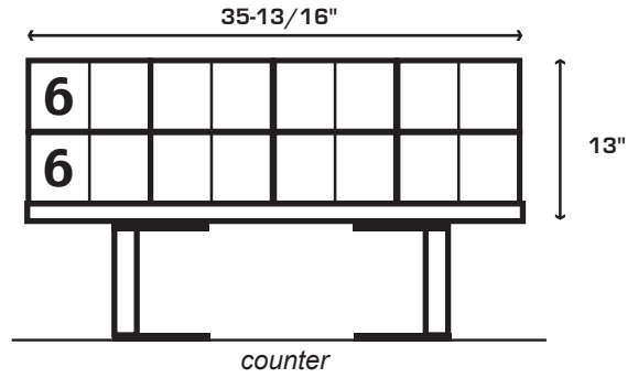
4 Wide Dual 6'' + 4 Wide Dual 6'' #OTS00664W
