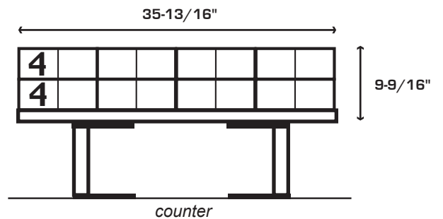
4 Wide Dual 4'' + 4 Wide Dual 4'' #OTS00444W
