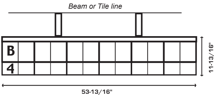
6 Wide Dual Bingo + 6 Wide Dual 4" #OCB00B46W #OCT00B46W
