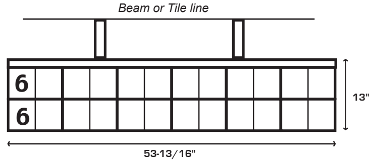
6 Wide Dual 6" + 6 Wide Dual 6" #OCB00666W #OCT00666W
